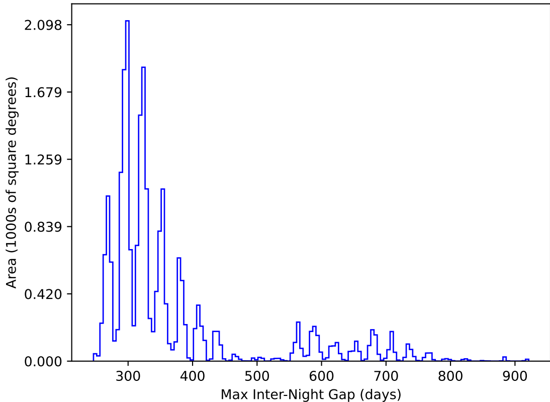
weather_cloudso1v3.4_10yrs All sky y band: Max Inter-Night Gap
