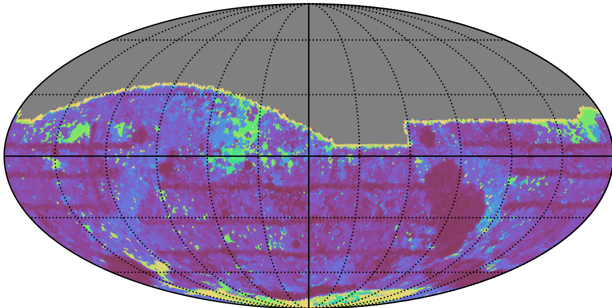
weather_cloudso1v3.4_10yrs All sky i band: Max Inter-Night Gap
