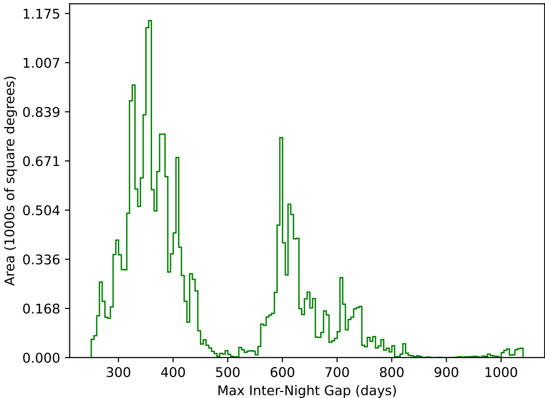
weather_cloudso1v3.4_10yrs All sky g band: Max Inter-Night Gap
