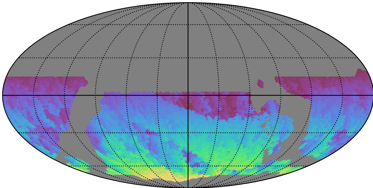
weather_cloudso1v3.4_10yrs WFD z band: Max HA
