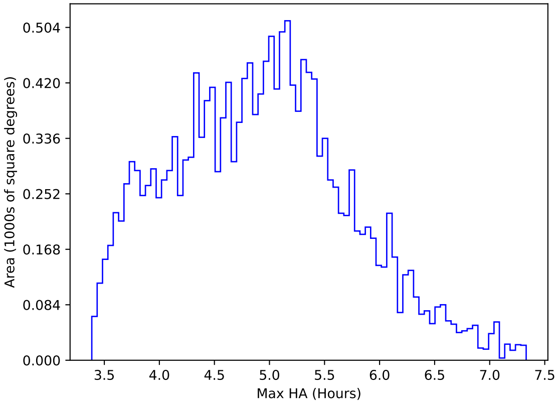
weather_cloudso1v3.4_10yrs WFD z band: Max HA
