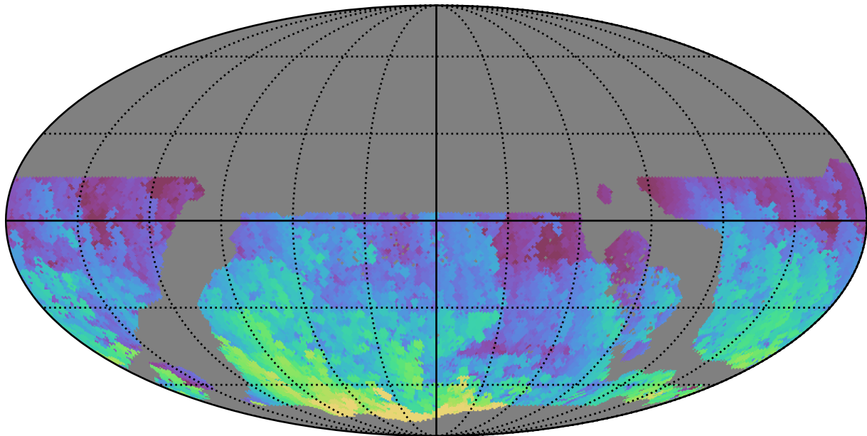
weather_cloudso1v3.4_10yrs WFD u band: Max HA
