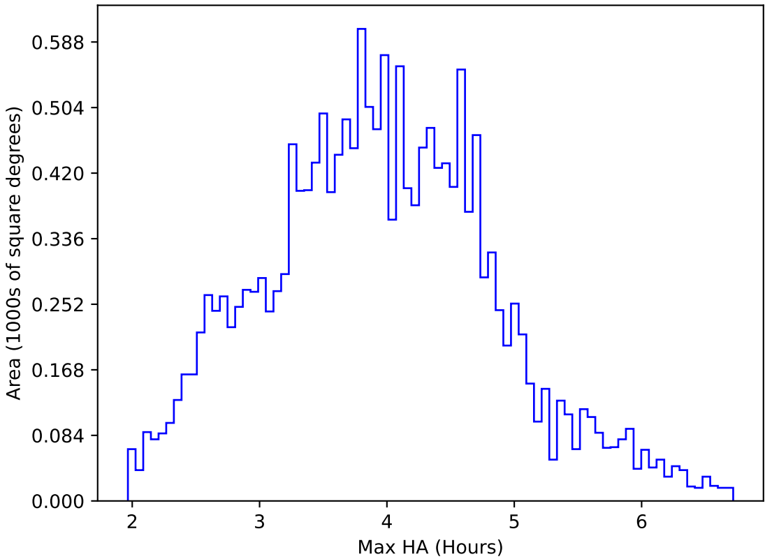
weather_cloudso1v3.4_10yrs WFD u band: Max HA
