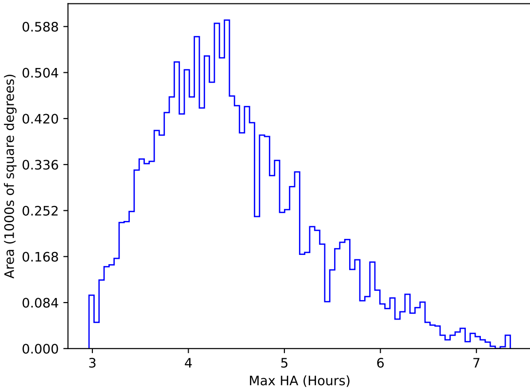
weather_cloudso1v3.4_10yrs WFD r band: Max HA
