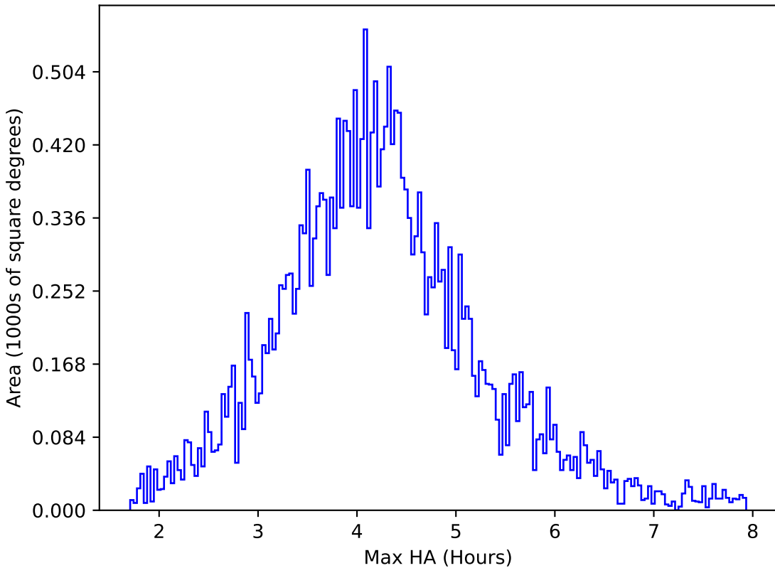
weather_cloudso1v3.4_10yrs All sky r band: Max HA
