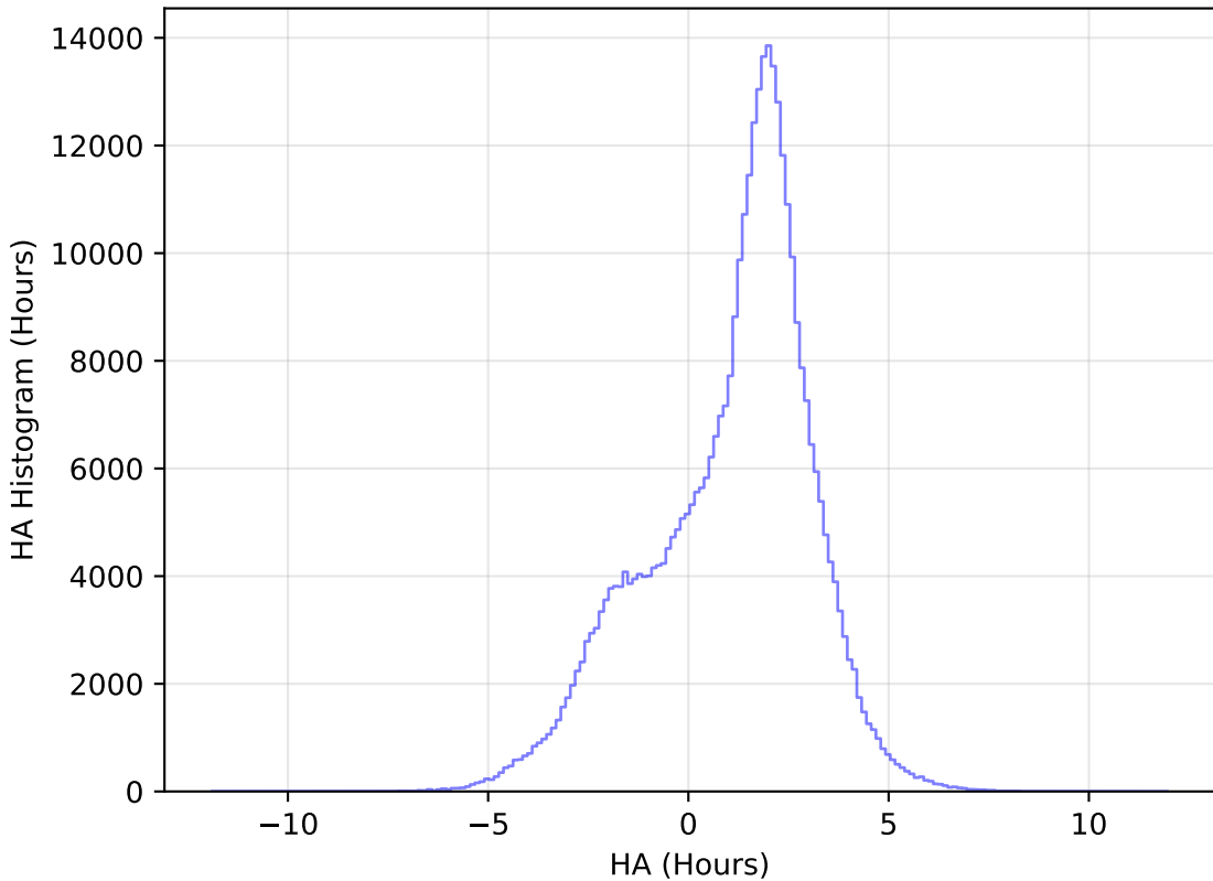
weather_cloudso1v3.4_10yrs WFD y band: HA Histogram
