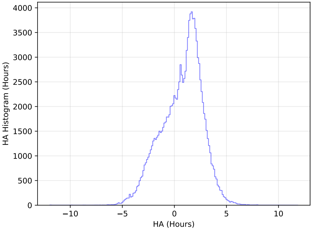
weather_cloudso1v3.4_10yrs WFD u band: HA Histogram
