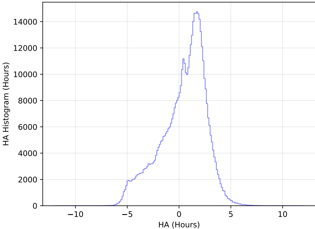
weather_cloudso1v3.4_10yrs WFD r band: HA Histogram
