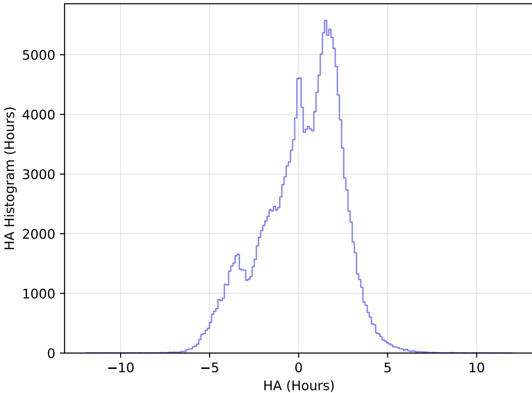
weather_cloudso1v3.4_10yrs WFD g band: HA Histogram
