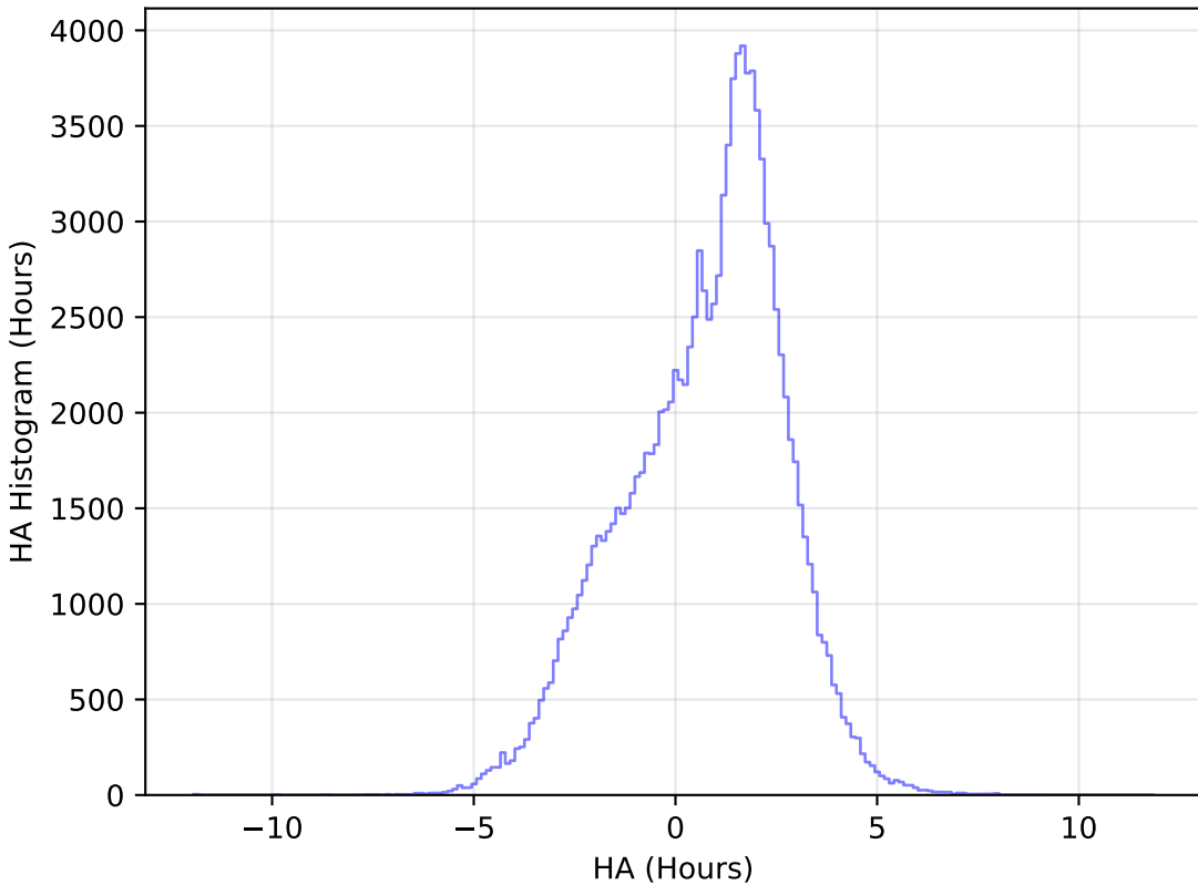
weather_cloudso1v3.4_10yrs All sky u band: HA Histogram
