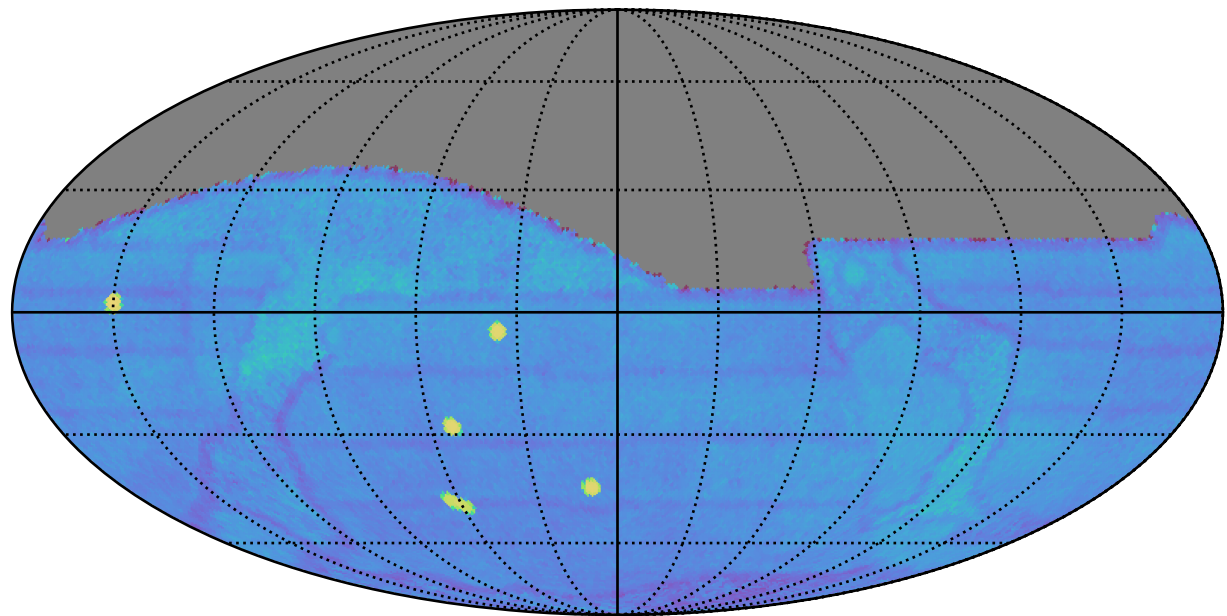
weather_cloudso1v3.4_10yrs gri All sky: Fraction of visits with a revisit < 60 min
