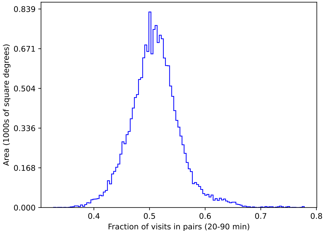
weather_cloudso1v3.4_10yrs gri WFD: Fraction of visits in pairs (20-90 min)
