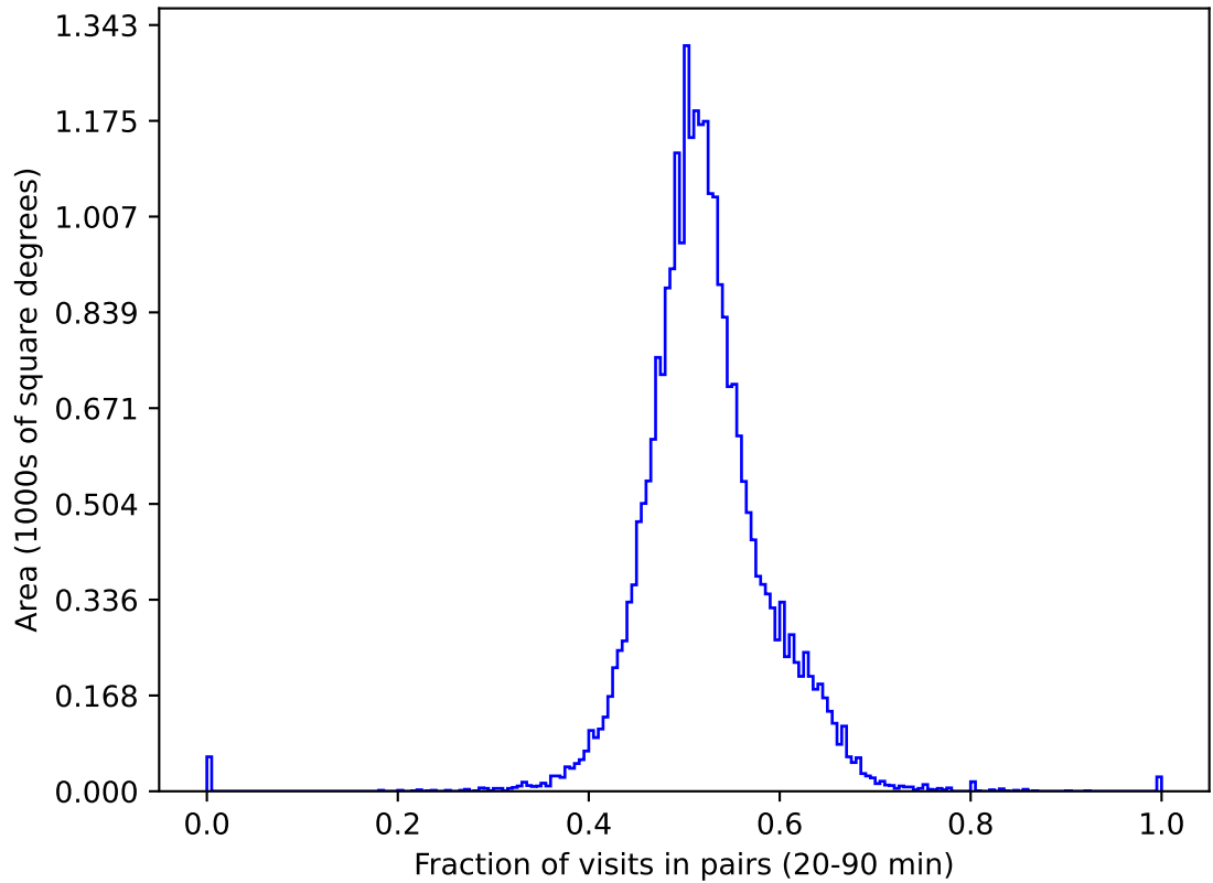
weather_cloudso1v3.4_10yrs gri All sky: Fraction of visits in pairs (20-90 min)
