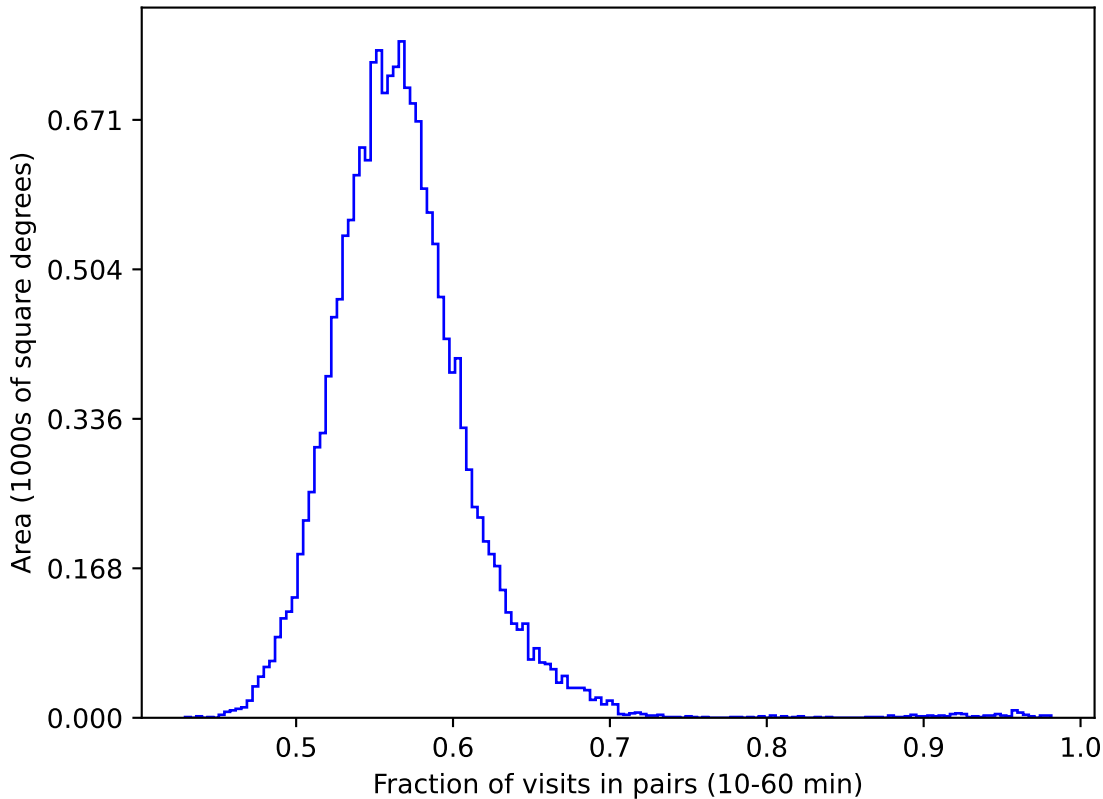
weather_cloudso1v3.4_10yrs gri WFD: Fraction of visits in pairs (10-60 min)
