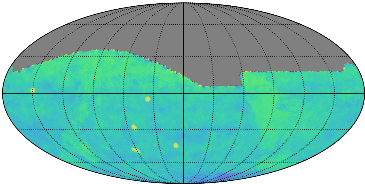
weather_cloudso1v3.4_10yrs gri All sky: Fraction of visits in pairs (10-60 min)
