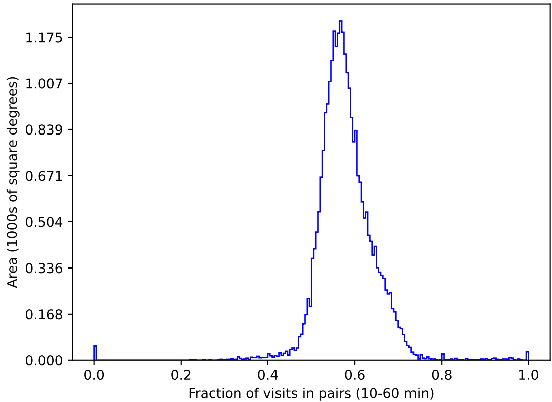
weather_cloudso1v3.4_10yrs gri All sky: Fraction of visits in pairs (10-60 min)
