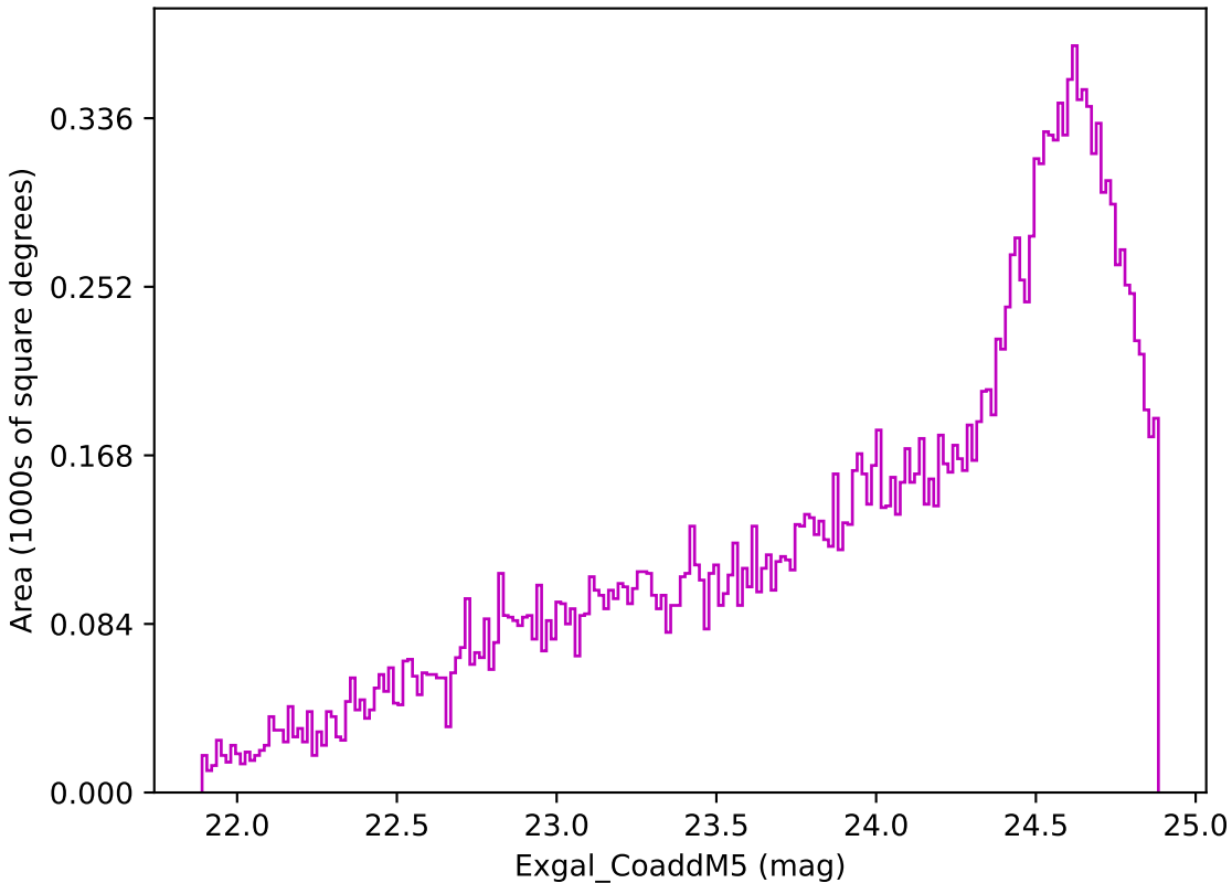
weather_cloudso1v3.4_10yrs Yr 3-4 z band: Exgal_CoaddM5
