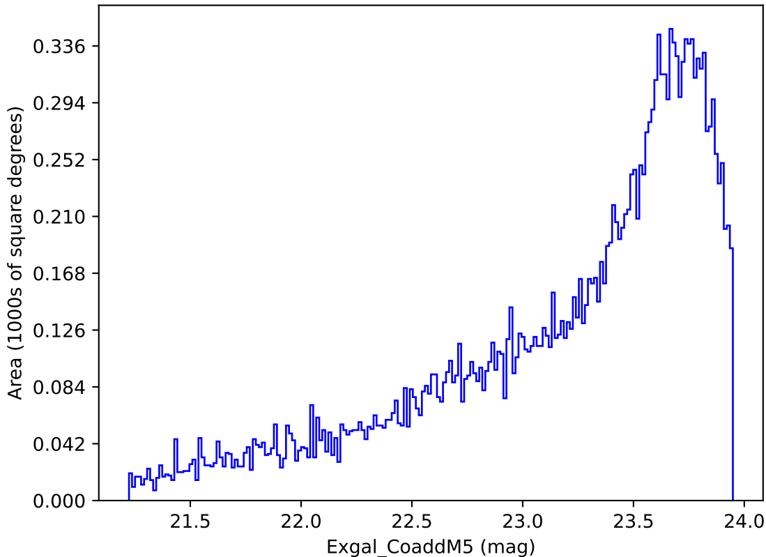
weather_cloudso1v3.4_10yrs Yr 3-4 y band: Exgal_CoaddM5
