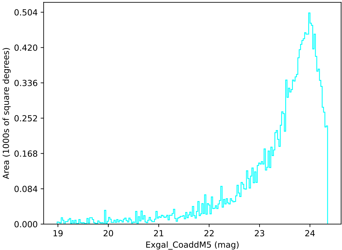
weather_cloudso1v3.4_10yrs Yr 3-4 u band: Exgal_CoaddM5
