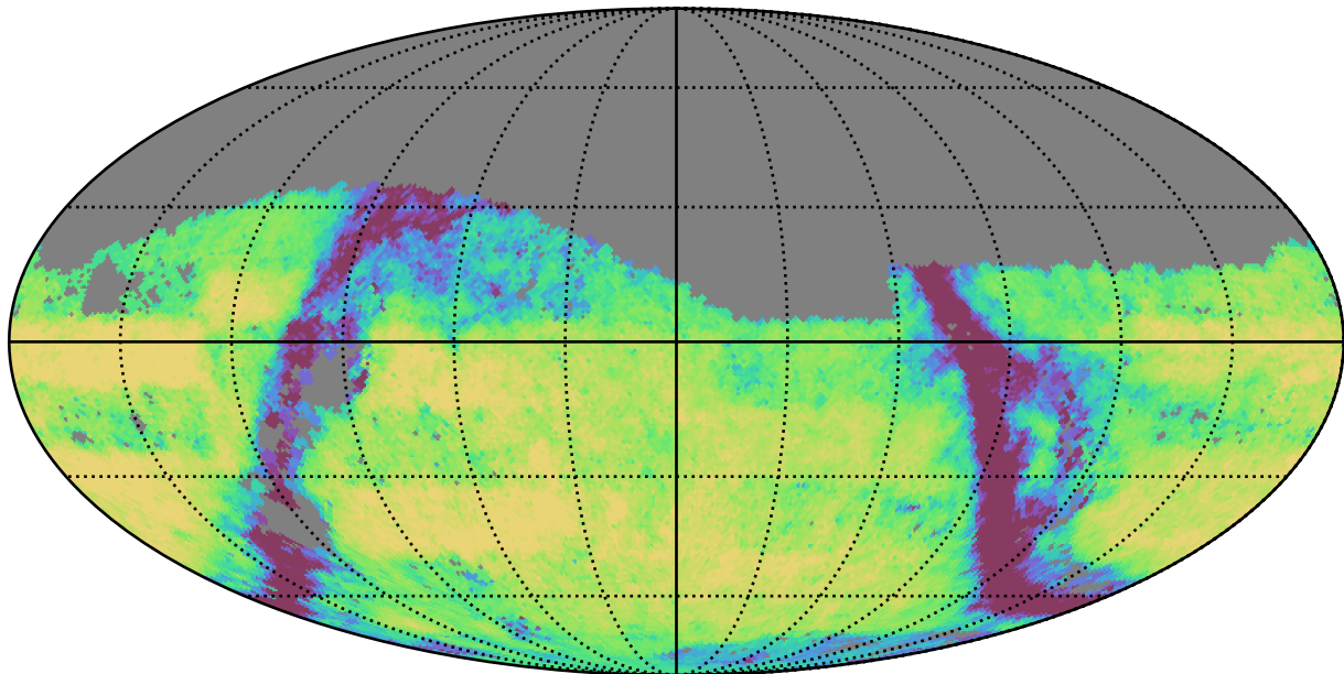
weather_cloudso1v3.4_10yrs Yr 3-4 g band: Exgal_CoaddM5
