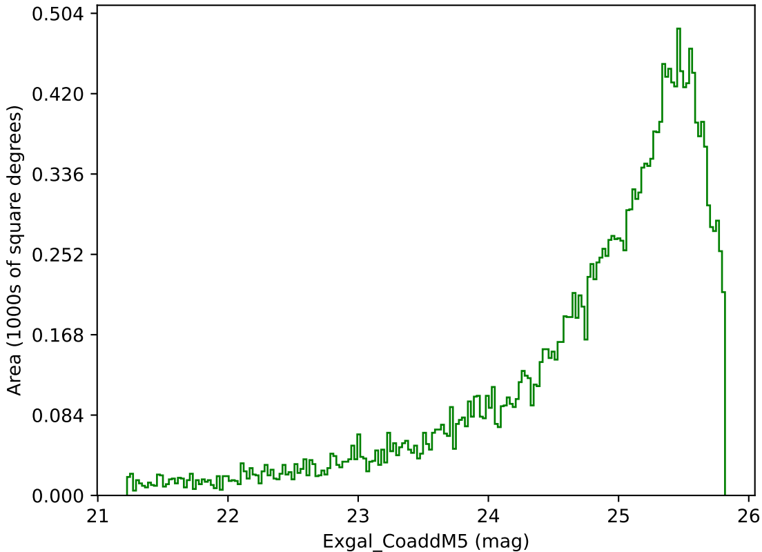
weather_cloudso1v3.4_10yrs Yr 3-4 g band: Exgal_CoaddM5
