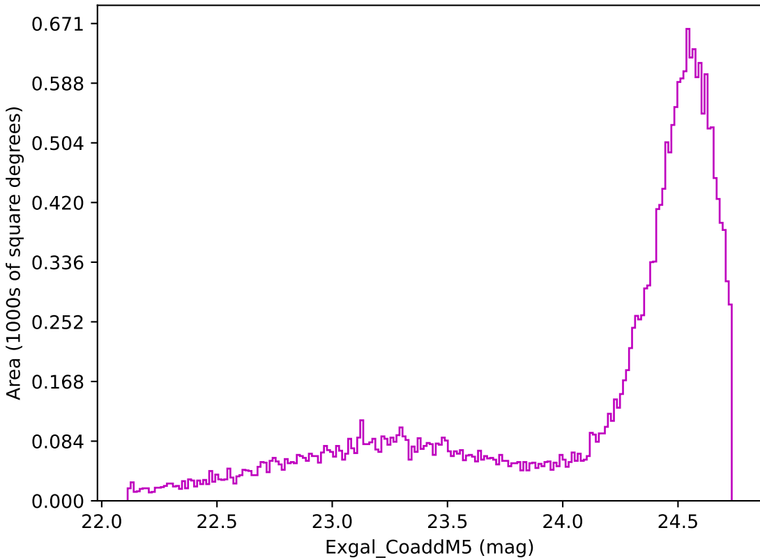
weather_cloudso1v3.4_10yrs Yr 1 z band: Exgal_CoaddM5
