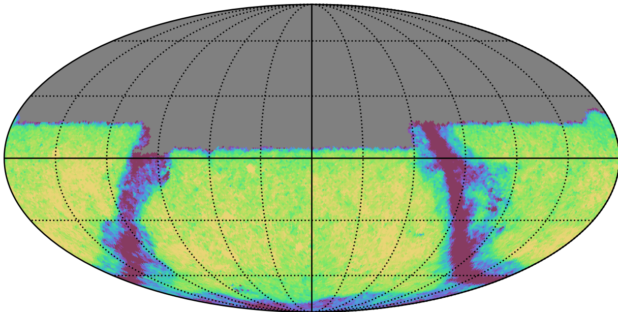
weather_cloudso1v3.4_10yrs Yr 1 y band: Exgal_CoaddM5
