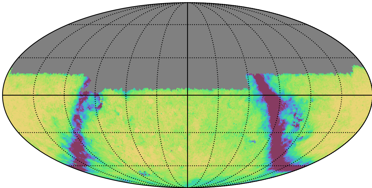
weather_cloudso1v3.4_10yrs Yr 1 u band: Exgal_CoaddM5
