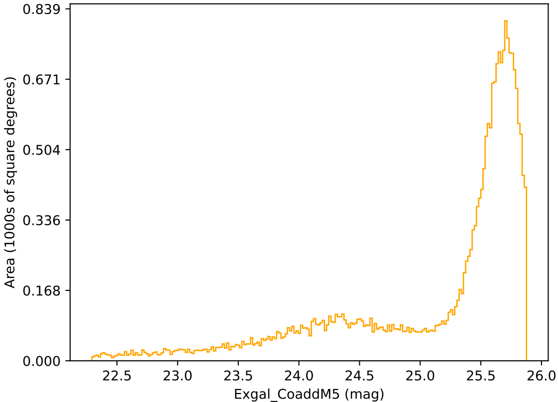
weather_cloudso1v3.4_10yrs Yr 1 r band: Exgal_CoaddM5
