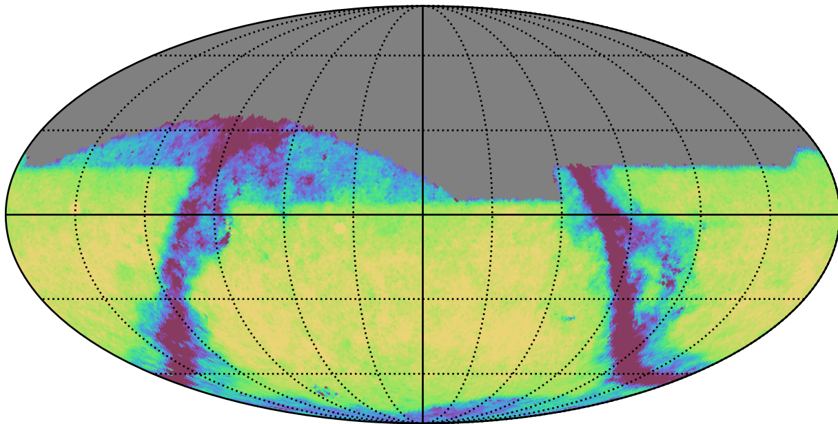
weather_cloudso1v3.4_10yrs Yr 1 i band: Exgal_CoaddM5
