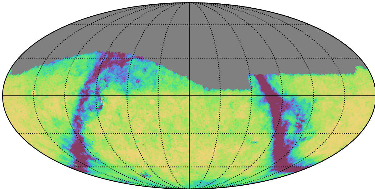
weather_cloudso1v3.4_10yrs Yr 1 g band: Exgal_CoaddM5
