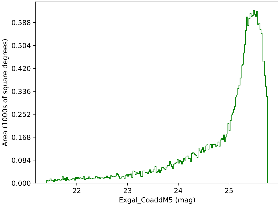
weather_cloudso1v3.4_10yrs Yr 1 g band: Exgal_CoaddM5
