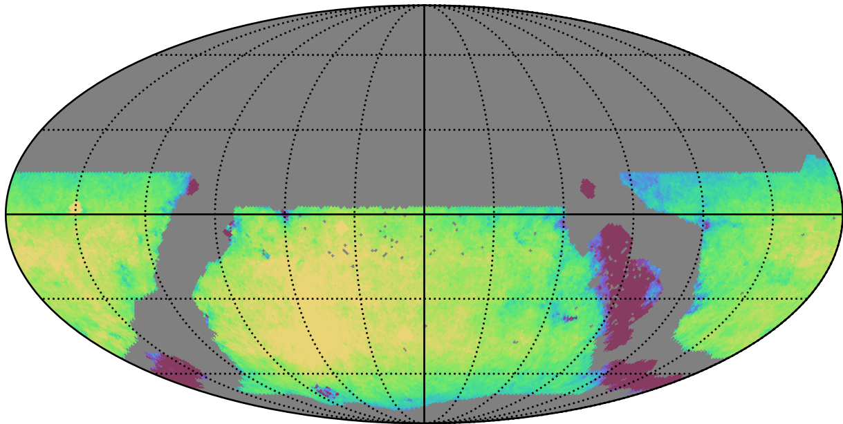
weather_cloudso1v3.4_10yrs WFD z band: Exgal_CoaddM5
