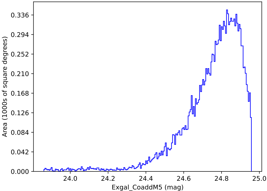
weather_cloudso1v3.4_10yrs WFD y band: Exgal_CoaddM5
