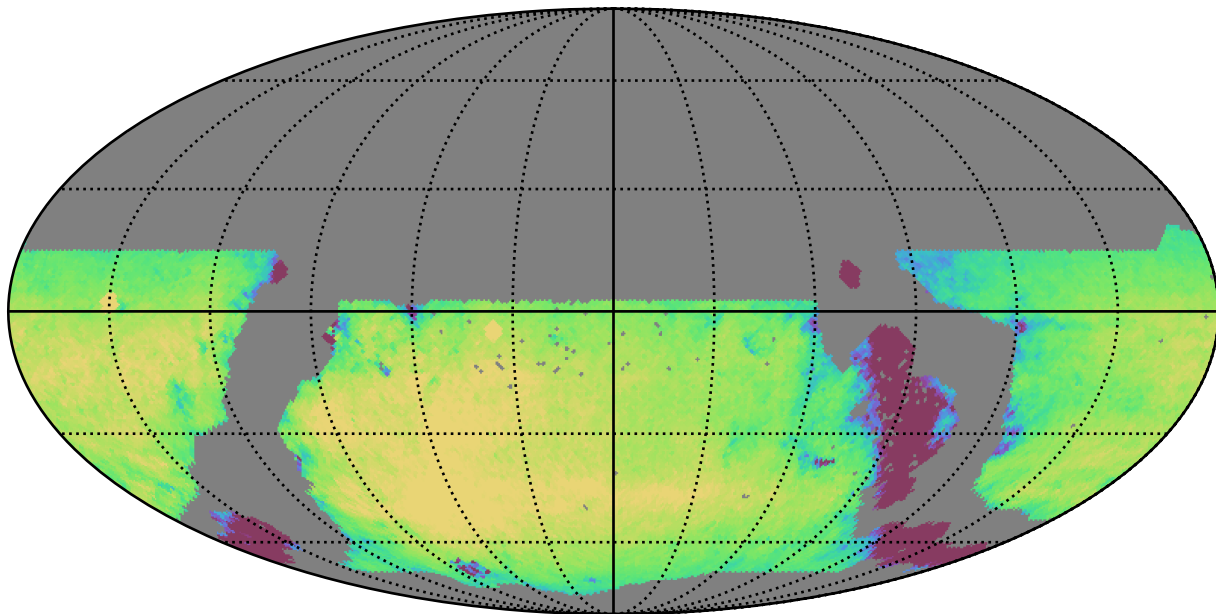
weather_cloudso1v3.4_10yrs WFD r band: Exgal_CoaddM5
