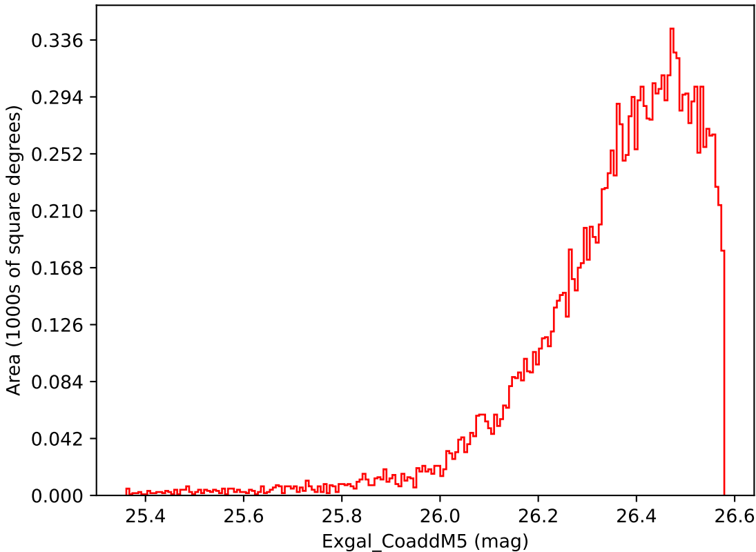
weather_cloudso1v3.4_10yrs WFD i band: Exgal_CoaddM5
