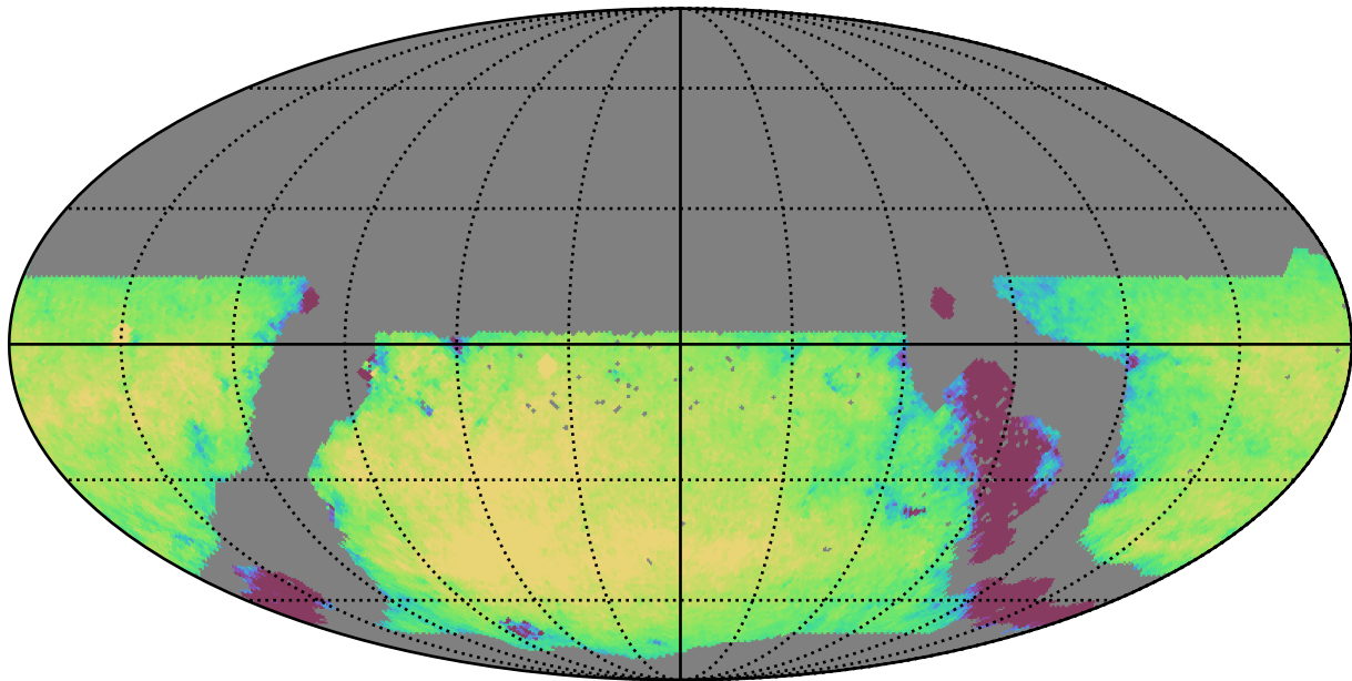
weather_cloudso1v3.4_10yrs WFD g band: Exgal_CoaddM5
