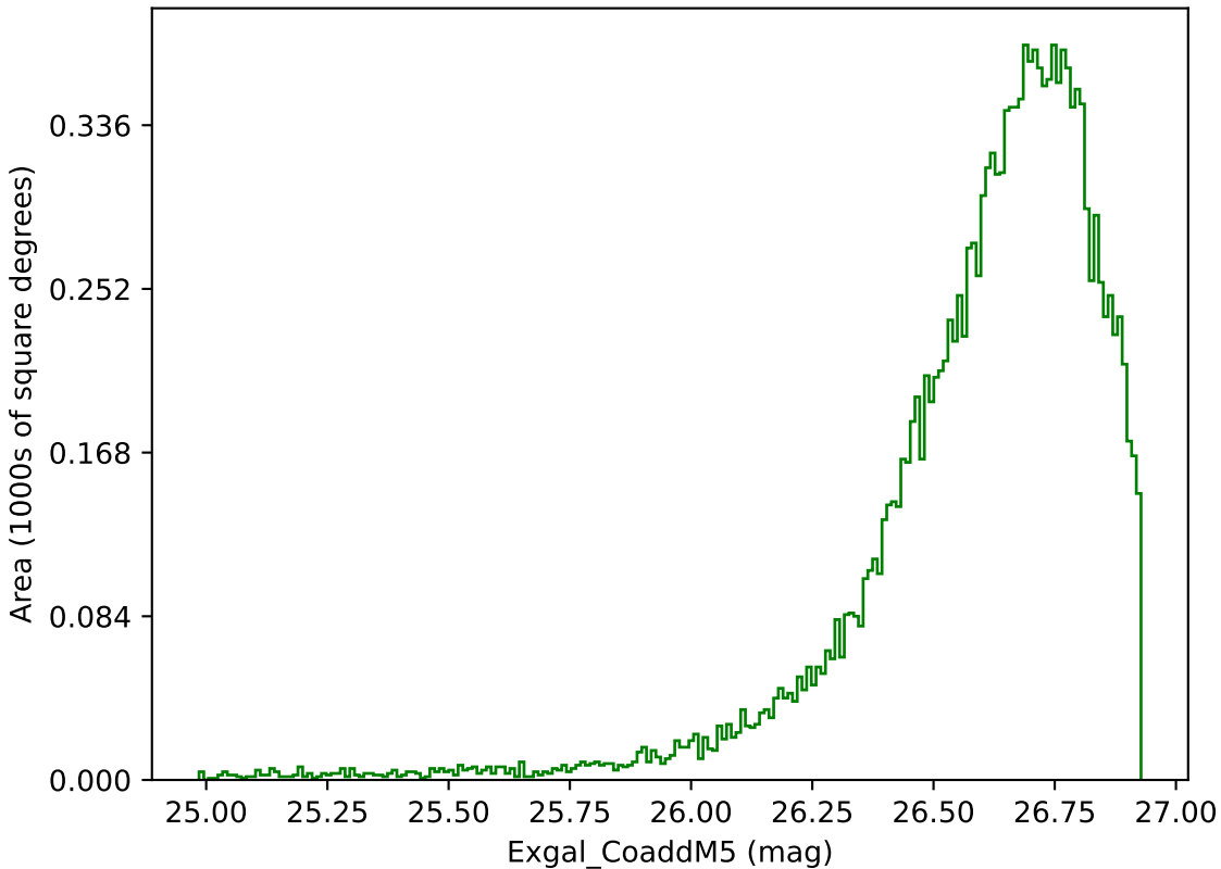
weather_cloudso1v3.4_10yrs WFD g band: Exgal_CoaddM5
