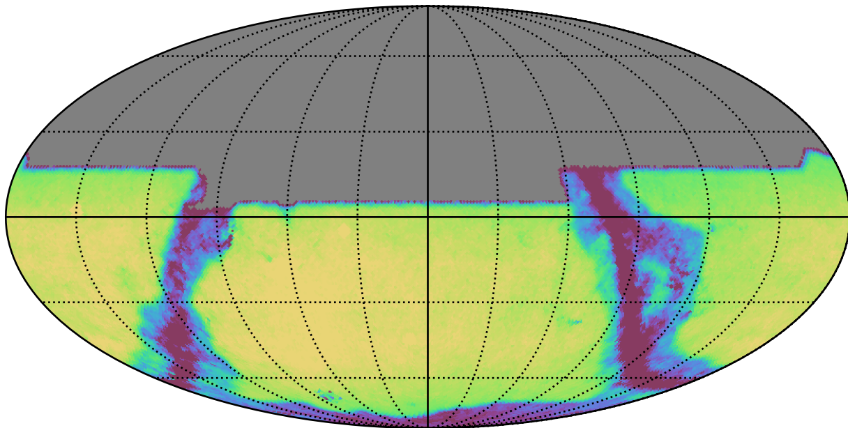
weather_cloudso1v3.4_10yrs All sky y band: Exgal_CoaddM5
