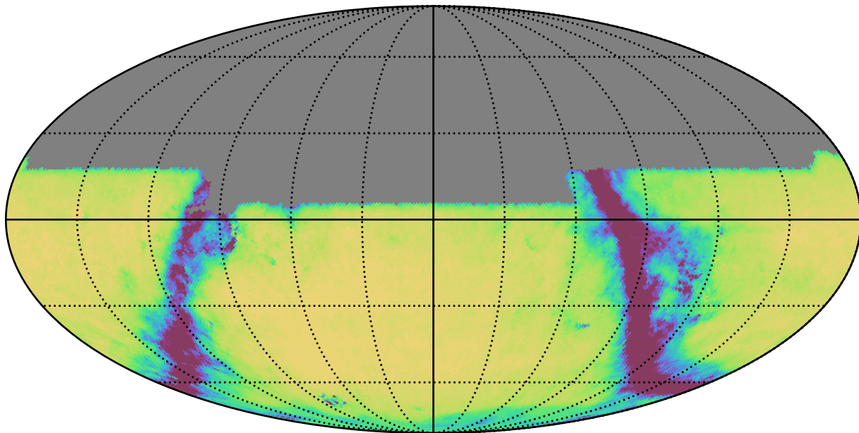
weather_cloudso1v3.4_10yrs All sky u band: Exgal_CoaddM5
