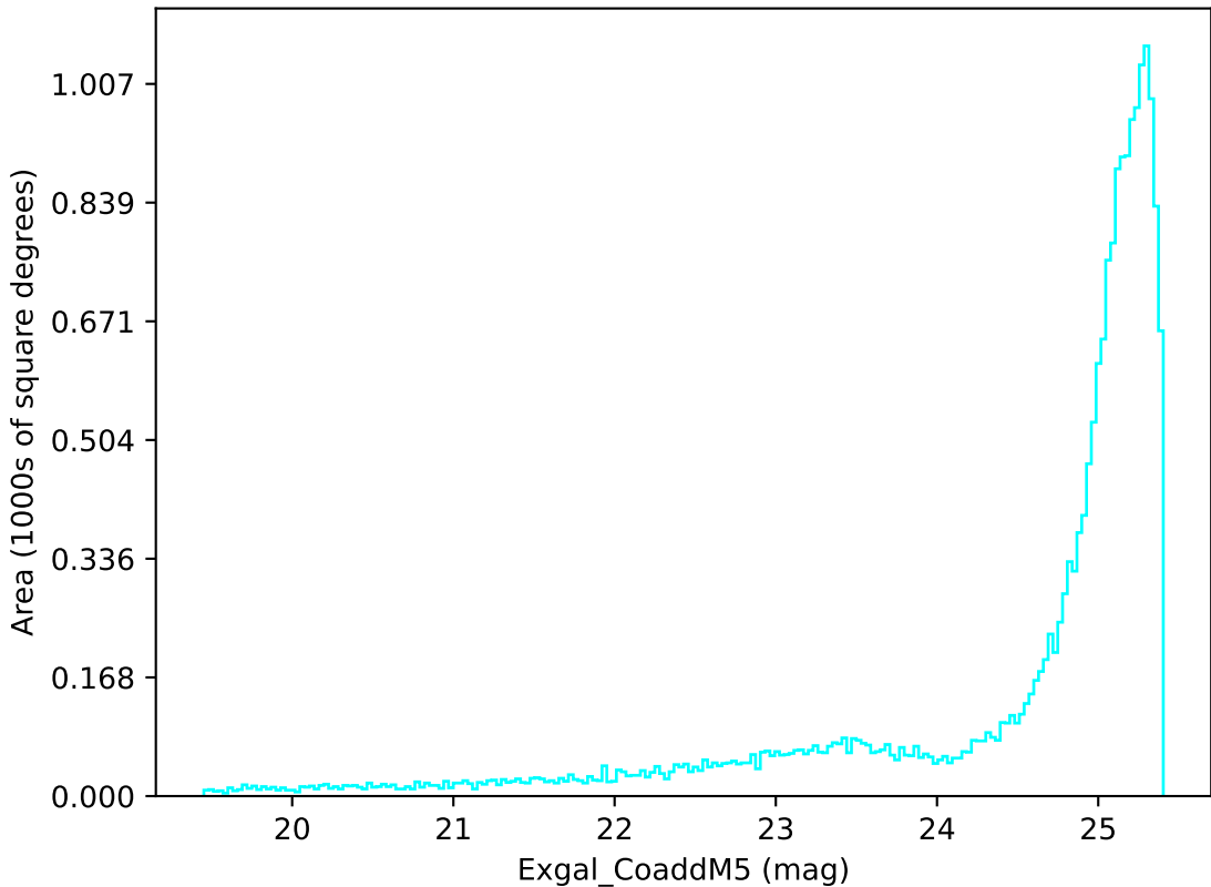
weather_cloudso1v3.4_10yrs All sky u band: Exgal_CoaddM5
