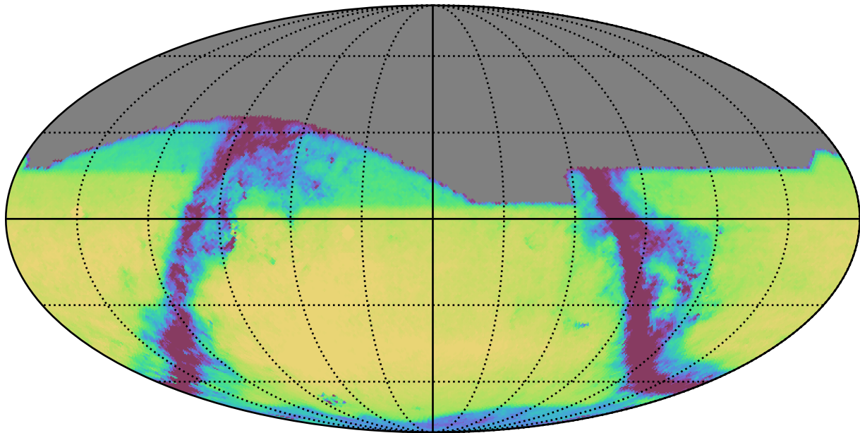
weather_cloudso1v3.4_10yrs All sky r band: Exgal_CoaddM5
