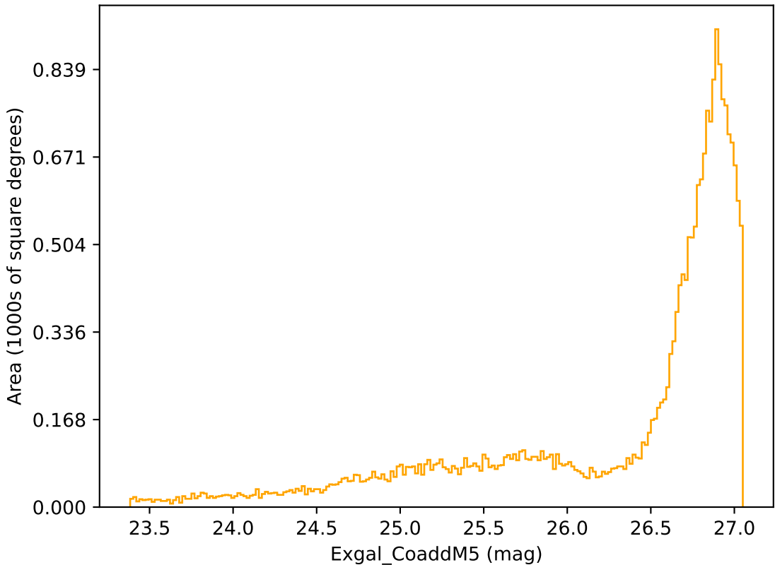
weather_cloudso1v3.4_10yrs All sky r band: Exgal_CoaddM5
