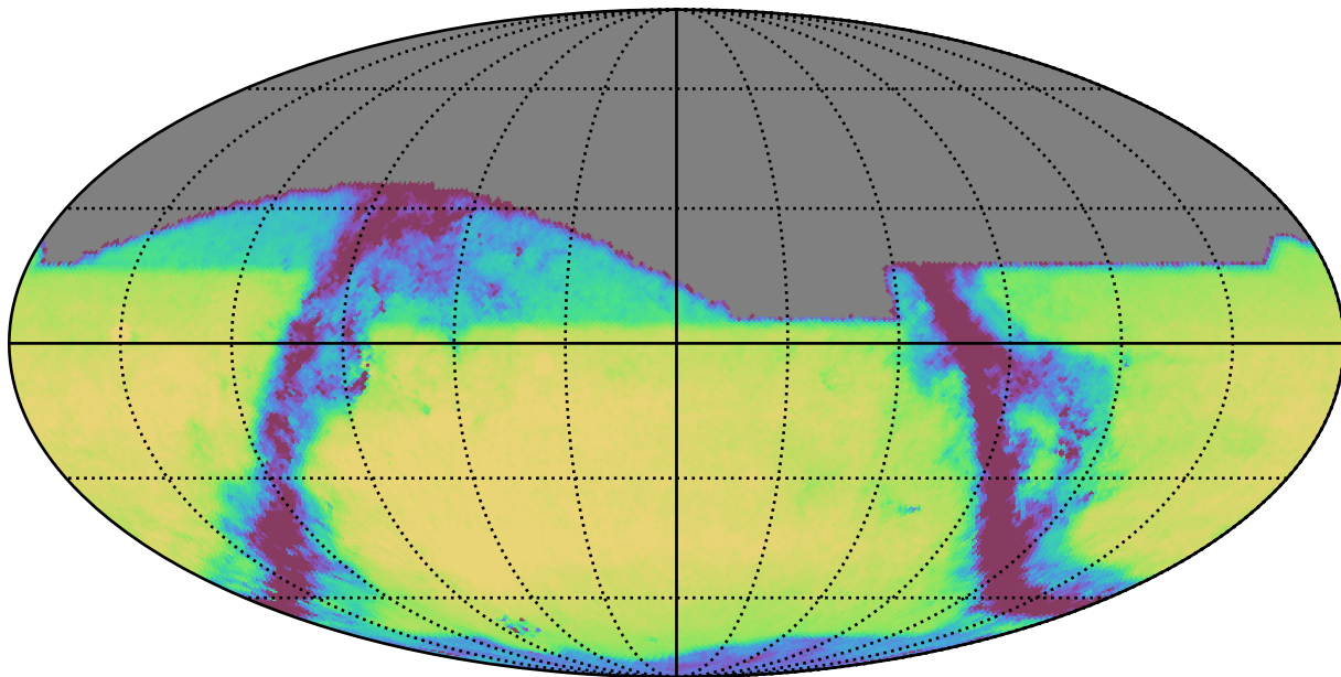
weather_cloudso1v3.4_10yrs All sky i band: Exgal_CoaddM5
