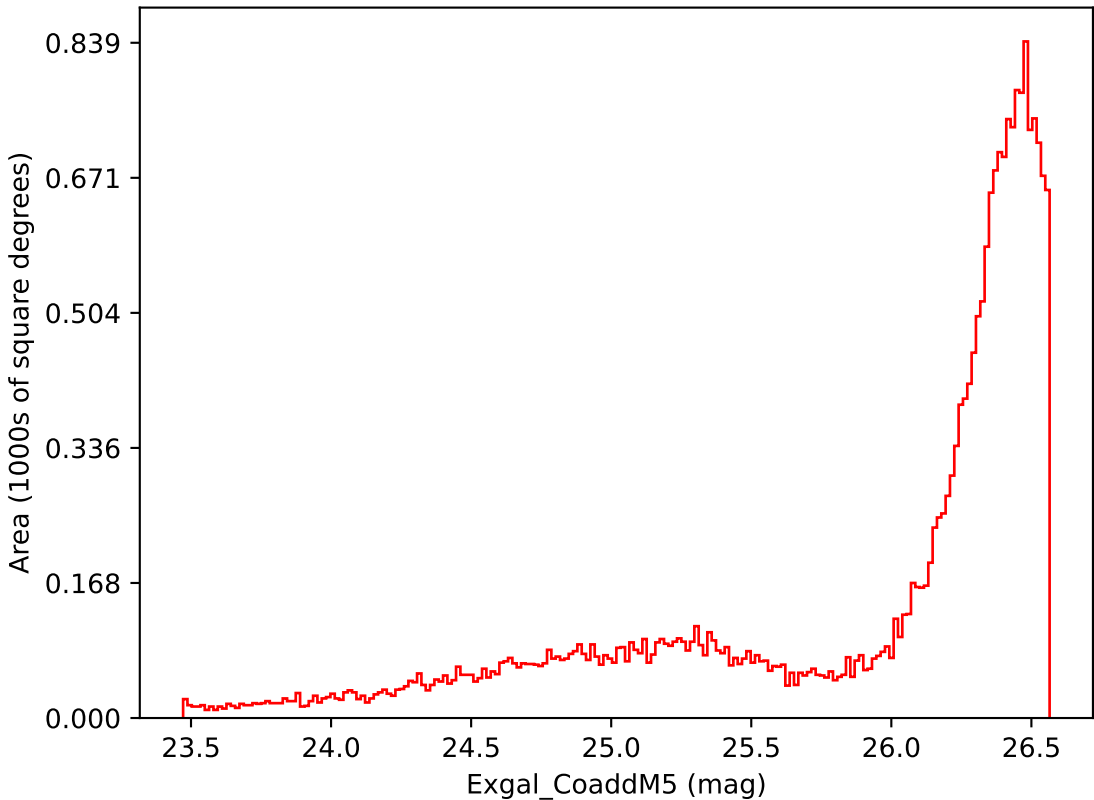
weather_cloudso1v3.4_10yrs All sky i band: Exgal_CoaddM5
