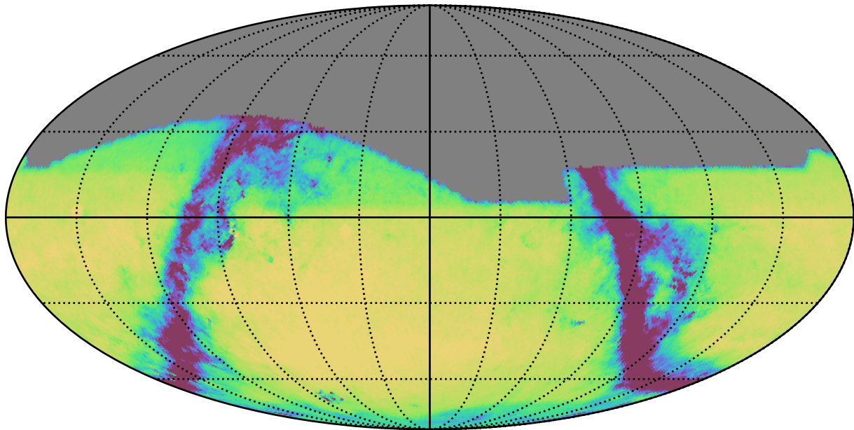
weather_cloudso1v3.4_10yrs All sky g band: Exgal_CoaddM5
