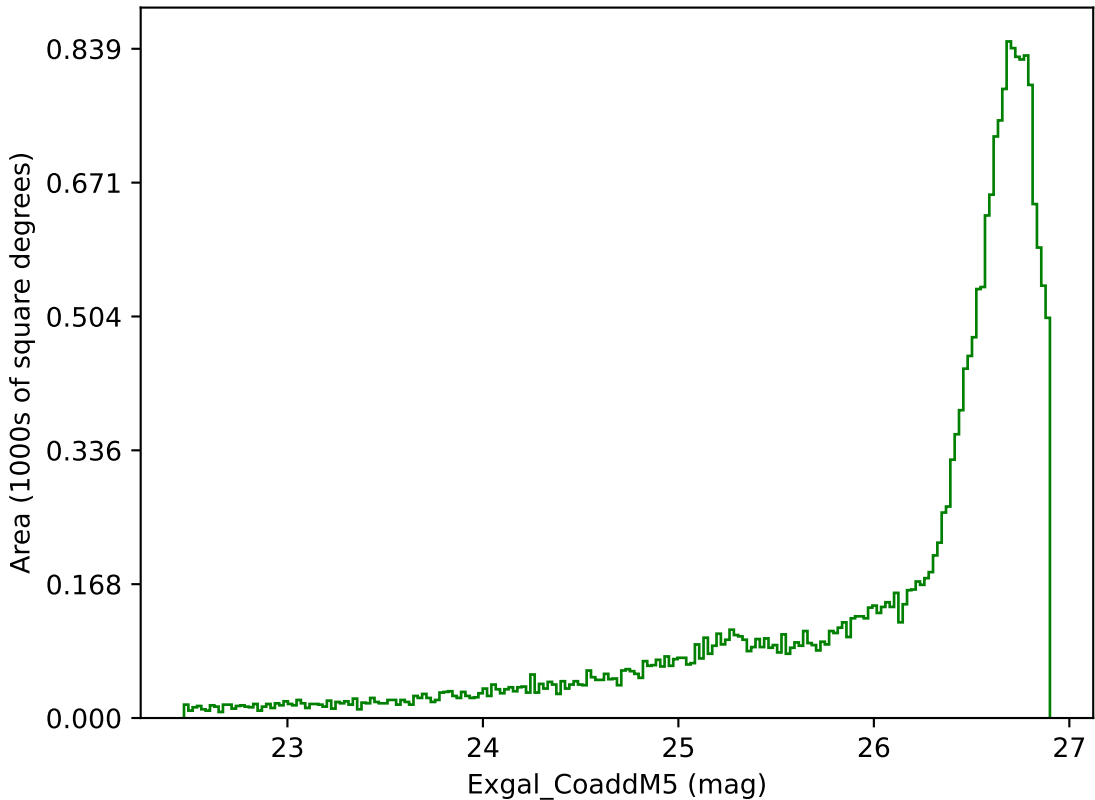
weather_cloudso1v3.4_10yrs All sky g band: Exgal_CoaddM5
