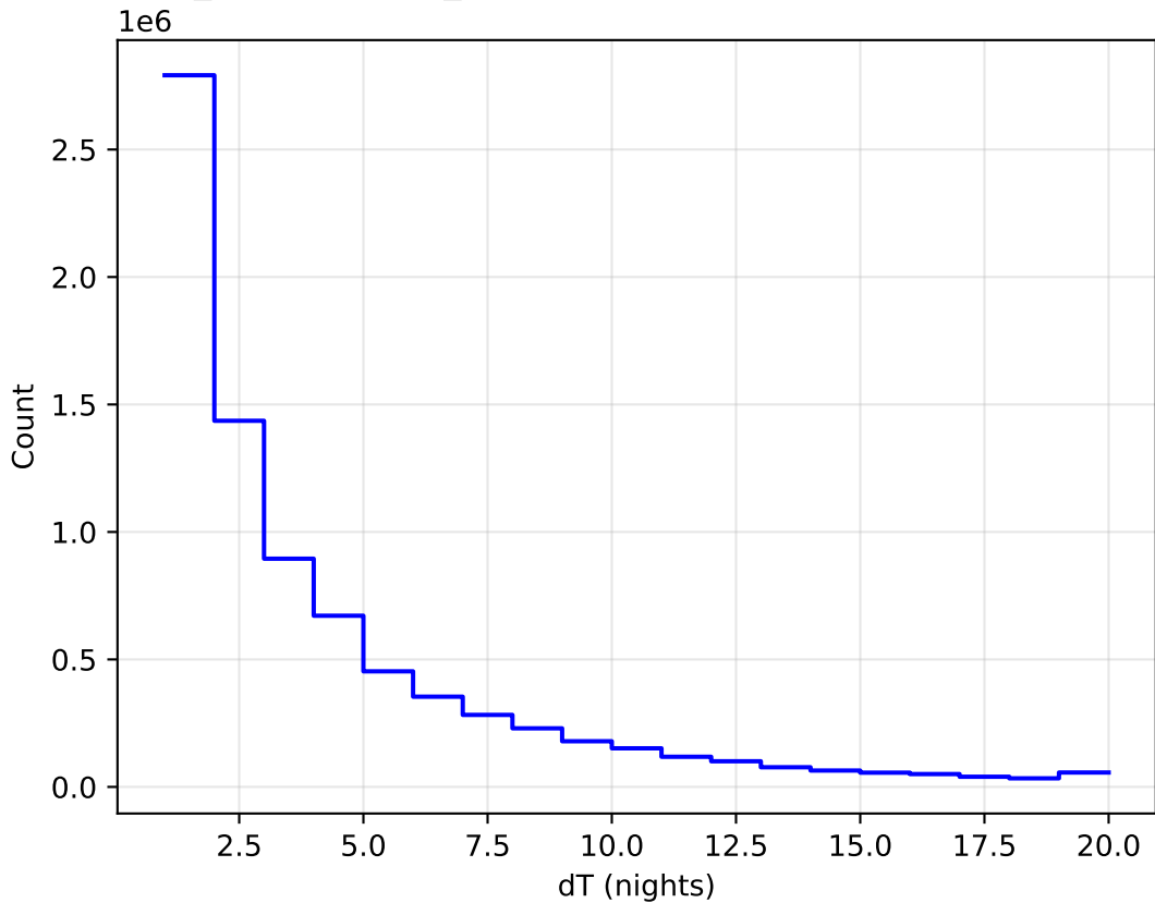
weather_cloudso1v3.4_10yrs WFD all bands: DeltaNight Histogram
