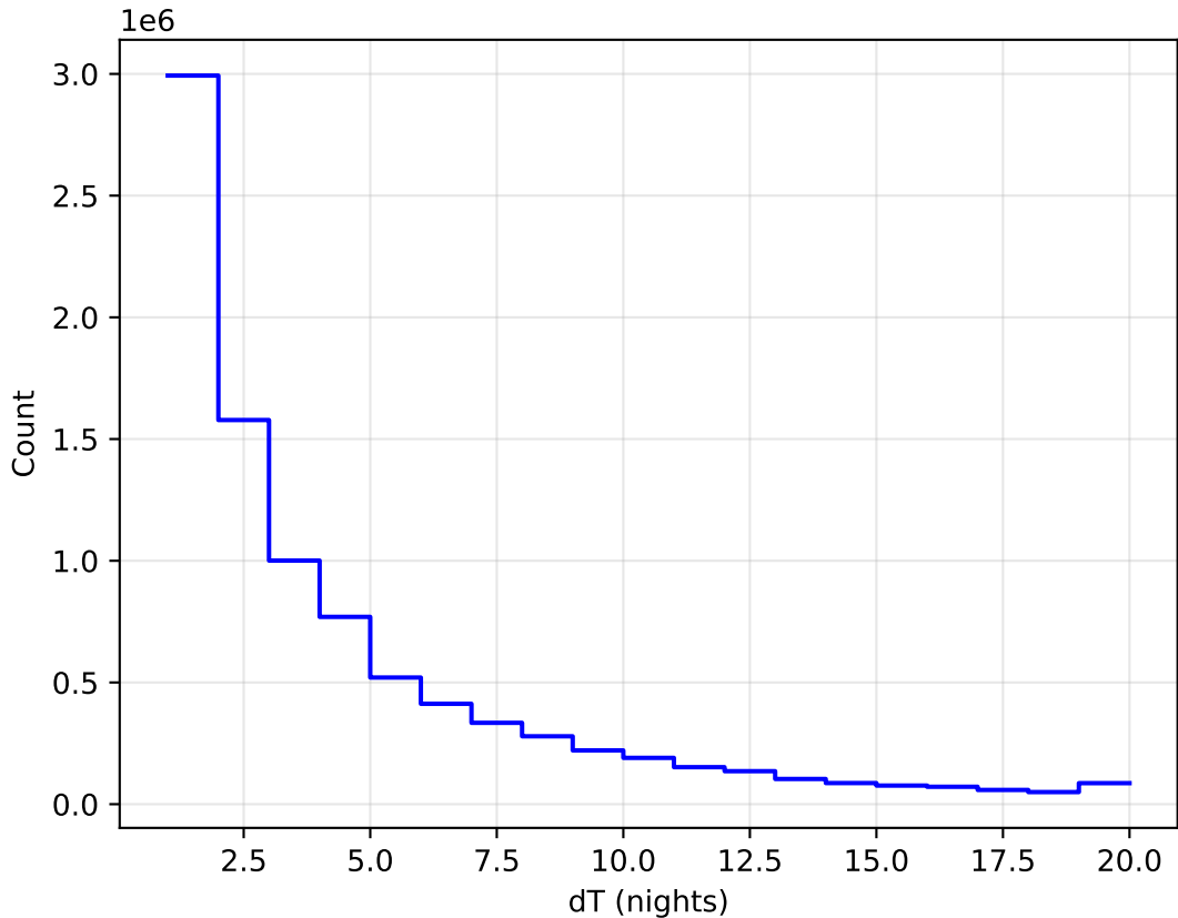
weather_cloudso1v3.4_10yrs All sky all bands: DeltaNight Histogram
