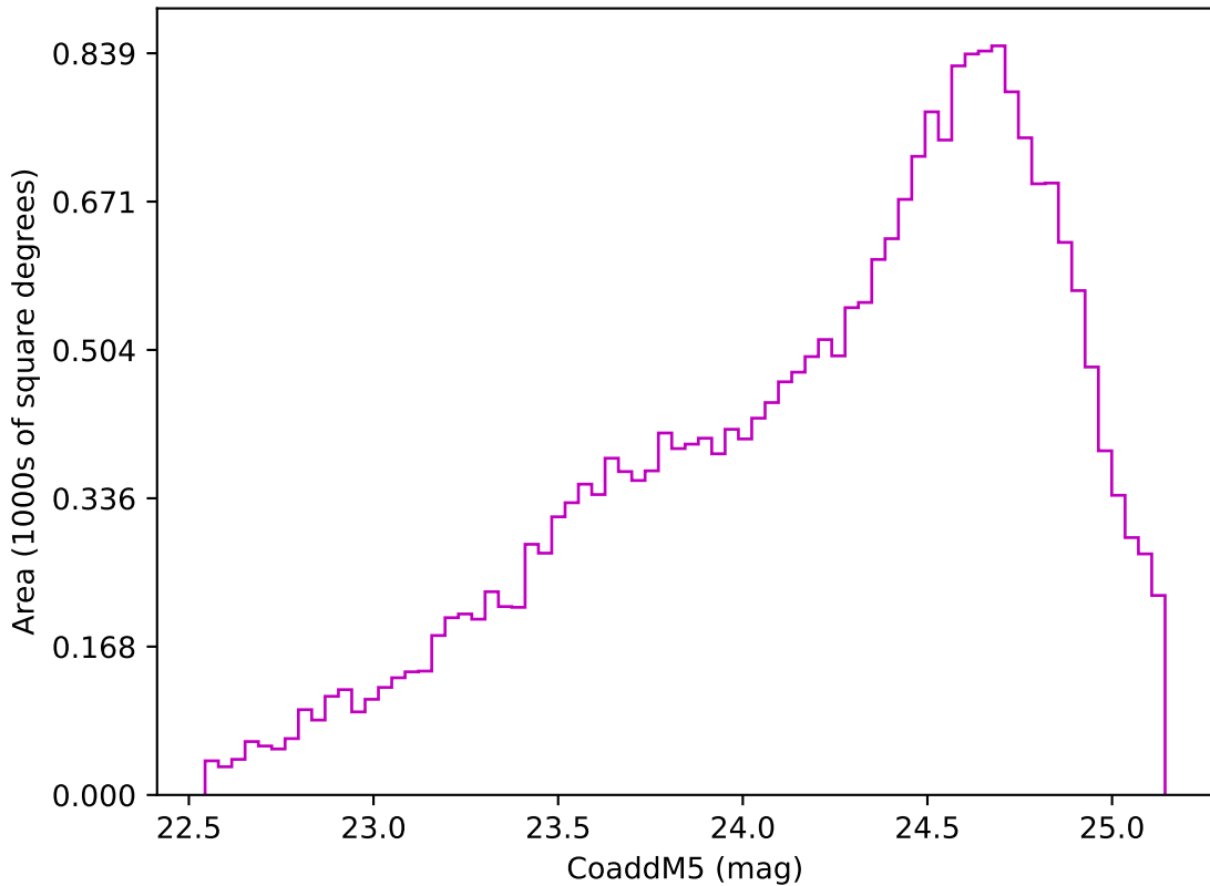
weather_cloudso1v3.4_10yrs Yr 3-4 z band: CoaddM5
